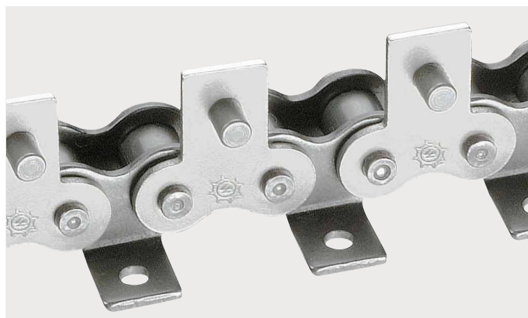
Roller chain stainless steel with bent or straight attachments on one side with pins Application: Materials handling
